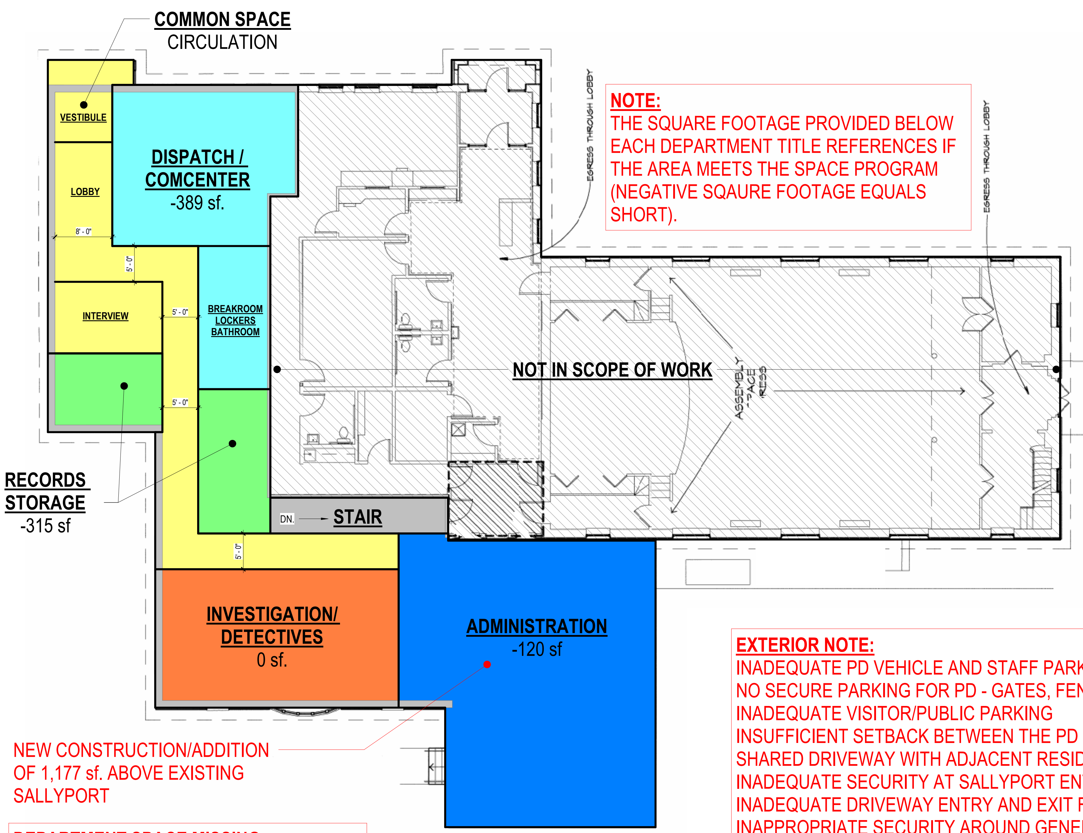
3 PROPOSED UPPER LEVEL FLOOR PLAN 1/8" = 1'-0"
